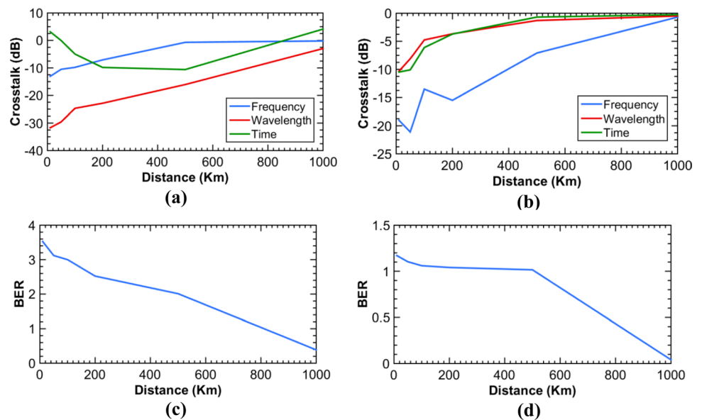
Fig. 9 Plot of the tested node outputs, where a crosstalk with distances for 1.10 \mu\text{m} , b crosstalk with distances for 1.30 \mu\text{m} , c BER for 1.10 \mu\text{m} , d BER for 1.30 \mu\text{m} . The BER results are not significant when the transmission rate is Tbit/s. The optimum shifted frequency is 2.9 GHz; the optimum shifted wavelength is 2.5 nm
