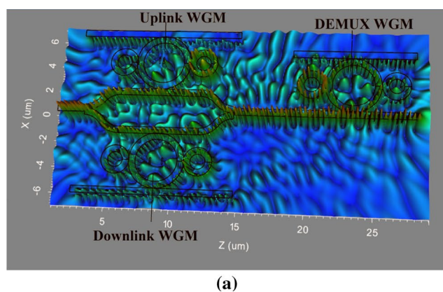
Fig. 2 The graphical result of WGMs using the Optiwave is observed at the uplink, downlink, and DEMUX WGM at 1.54\ \mu\text{m} , where a formation of WGMs in the system, b electric field distribution within the system. The used parameters are given in Table-1, which are also applied in MATLAB. The center wavelengths shift to Bragg wave-
