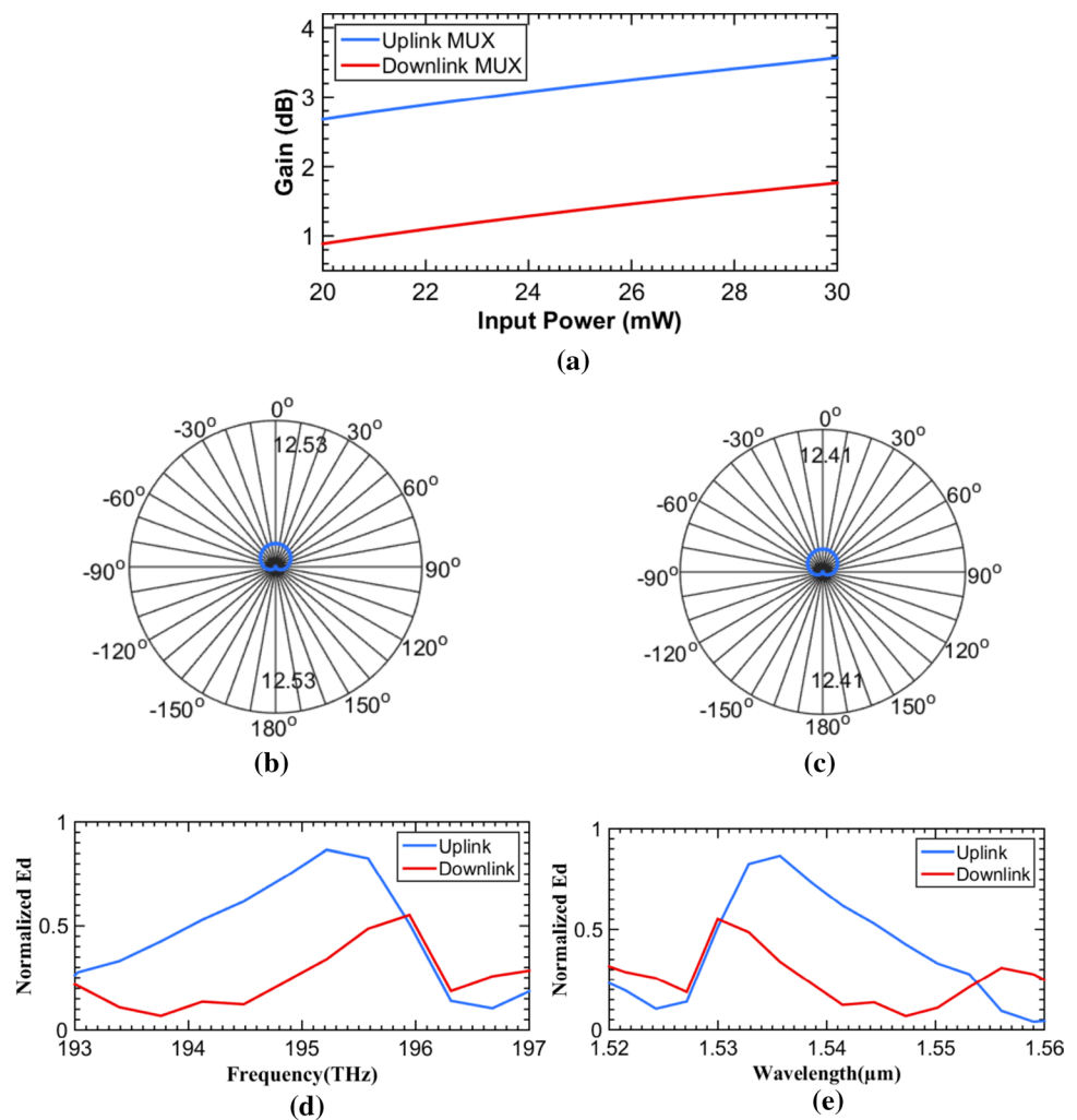
Fig. 7 Plot of the antenna profiles, where a gain, b directivity of uplink, c directivity of downlink, (d) WiFi uplink and downlink frequency bands, 1 LiFi uplink and downlink wavelength bands. The center frequency and wavelength are 195.2 THz and 195.9 THz and, 1.535 \mu\text{m} and 1.530 \mu\text{m} for uplink and downlink, respectively
